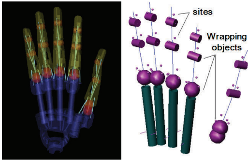
Fig. 10. Modeling of the robotic hand. Left : Kinematic model of the robotic hand visualized in OpenGL. Right : The model of the tendon paths.
